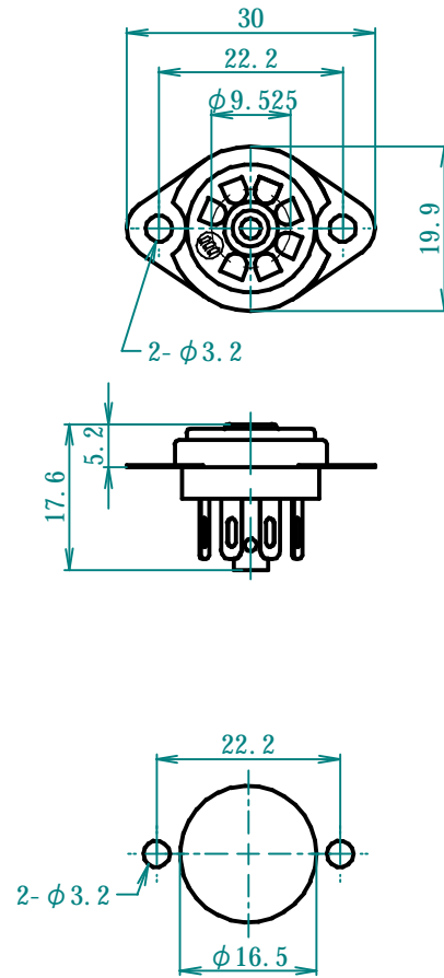
Mounting Hole
