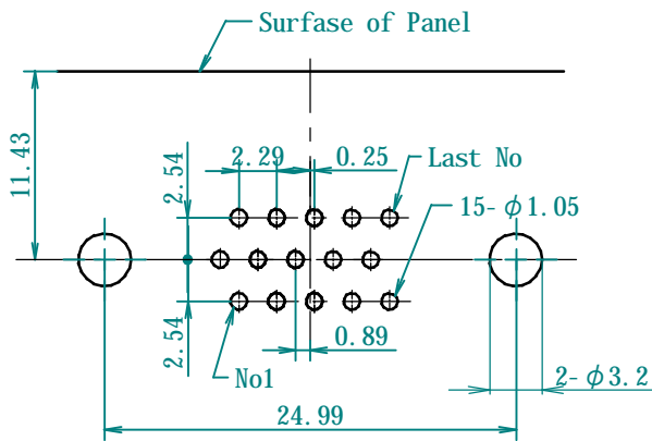
Hole Layout (Bottom View)
