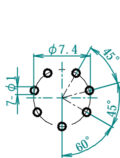
Mounting Hole Recommended P.C. Board thickness t1.6mm
