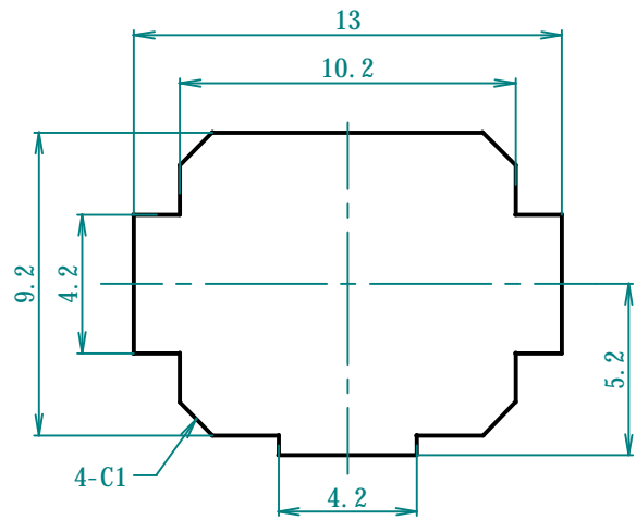
Panel Mounting Hole
